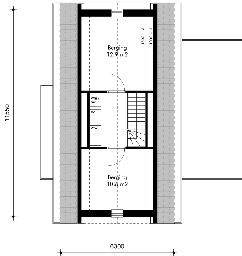
Zolder
